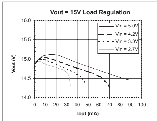
Figure 4. 15V Output Load Regulation
